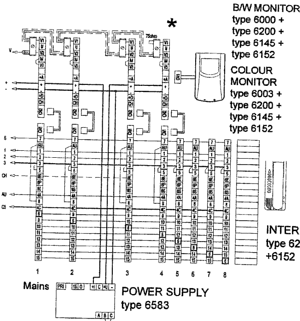
Fig. 3 Four monitors and four intercommunicating interphones.
