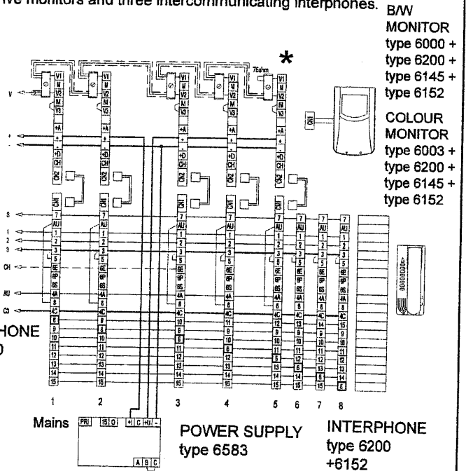
Fig. 4 Five monitors and three intercommunicating interphones.
