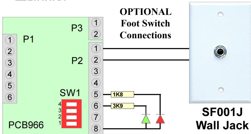
PC Board on Rear of SS200 series Master Station
