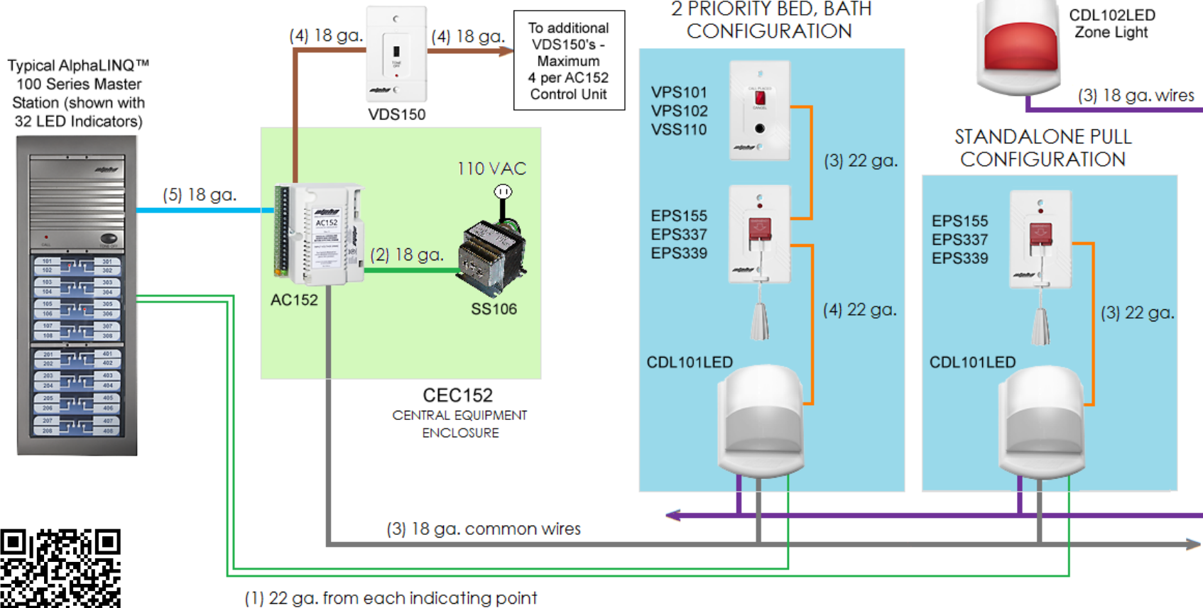
This diagram represents a typical basic system. For more specific details and variations, please refer to the AlphaLINQ™ 100 Series Installation & Operation Manual AWD183.
