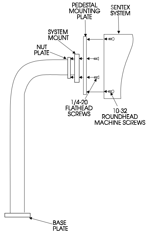
Diagram of the Pedestal Mounting Plate Installation
