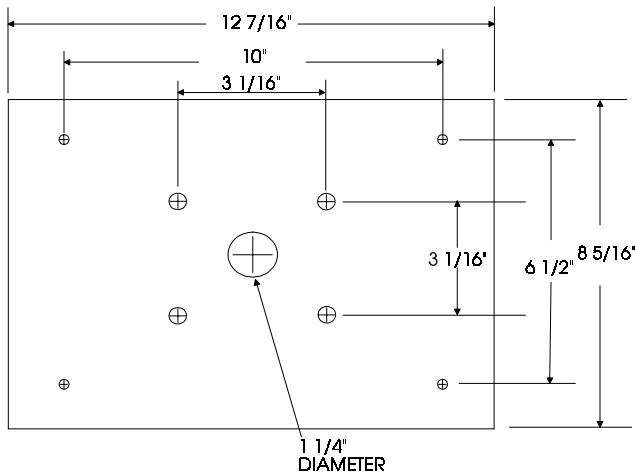
Dimensions of the Pedestal Mounting Plate (3/16" thick)
