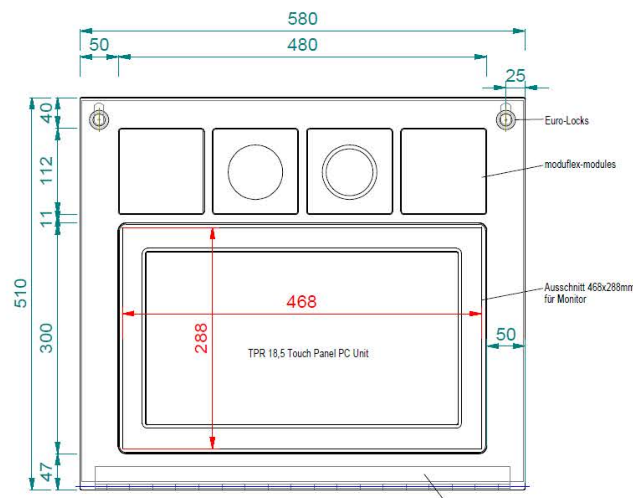
front view
