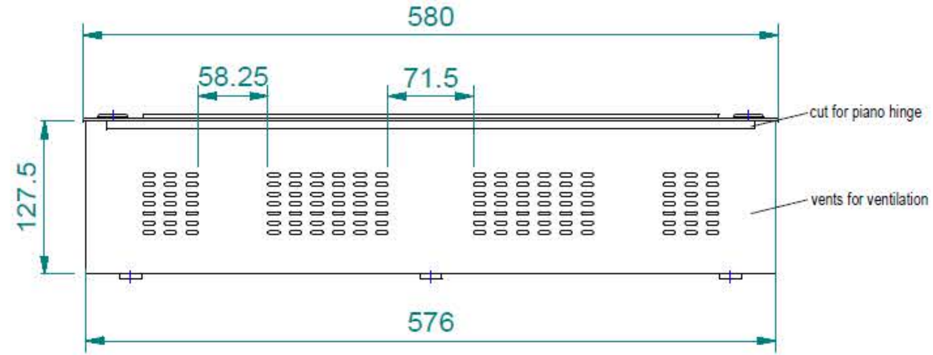
bottom view
