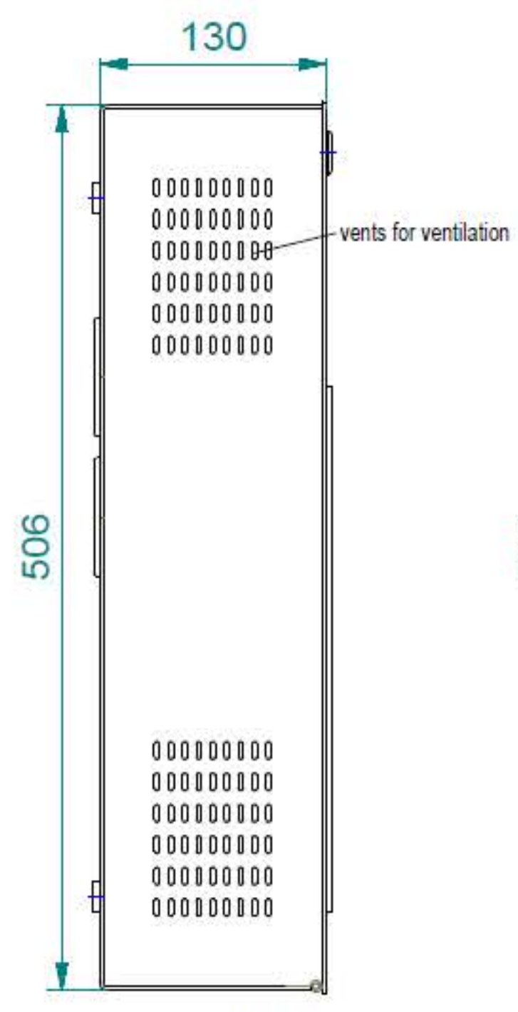
left-side view
