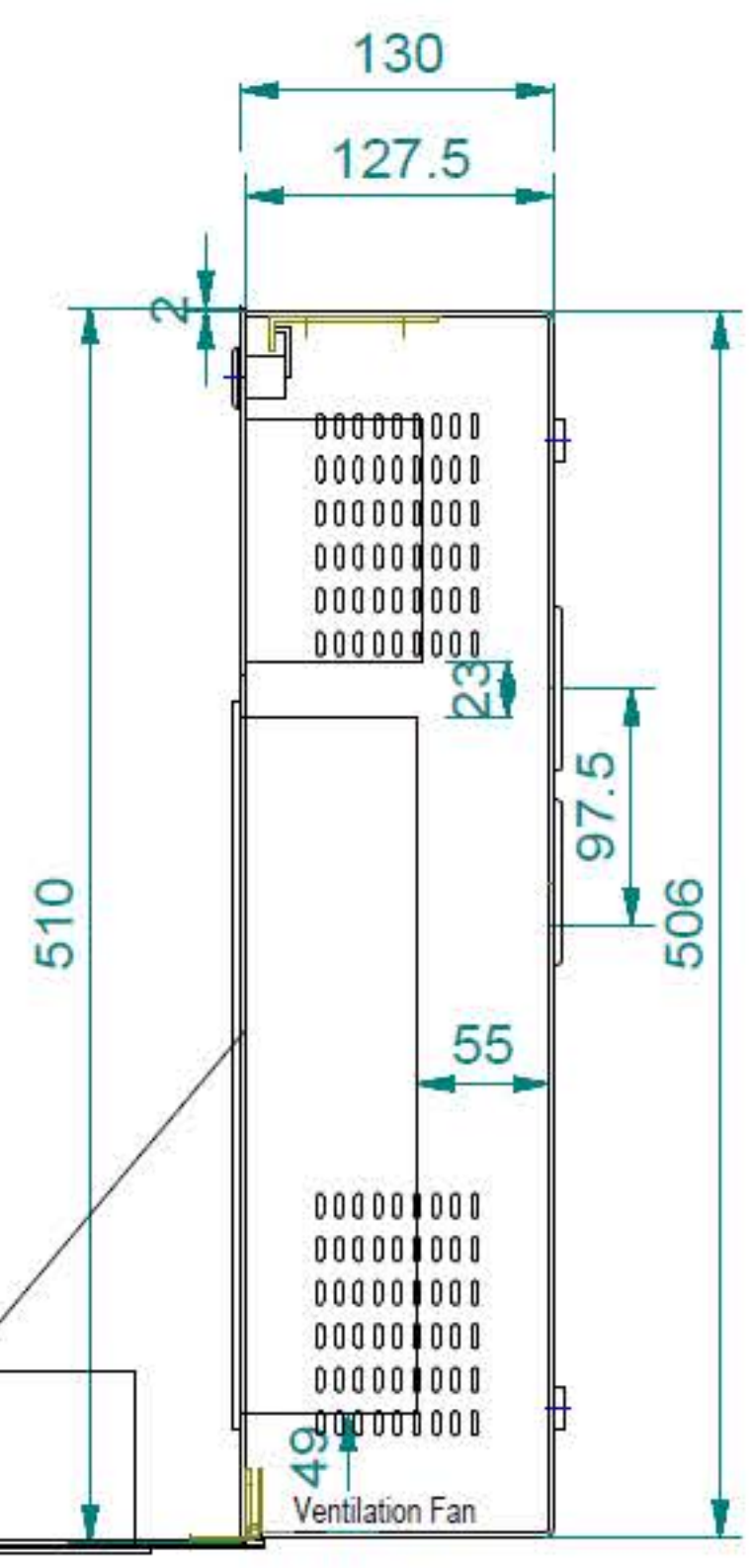
right-side view
